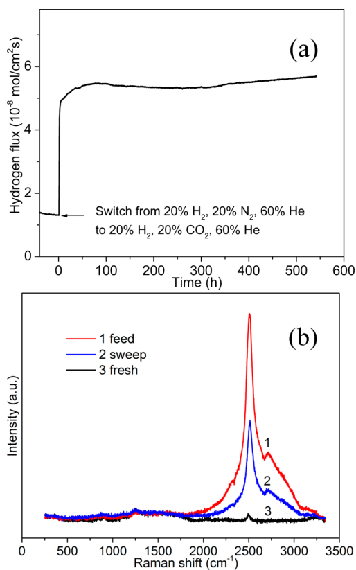
Figure 7. (a) Time dependence of hydrogen flux and moisture content in 20% H_2 , 20% CO_2 , and 60% He at 900 °C. Membrane thickness is 0.4 mm. (b) Raman spectra of Ni-BZCYYb membrane before and after test in 20% CO_2 at 900 °C for 540 h.
