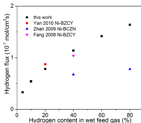
Figure 3. Dependence of hydrogen flux of a 0.4 mm thick membrane on hydrogen content in feed gas containing 3% H 2 O. Literature data are added for the ease of comparison.
